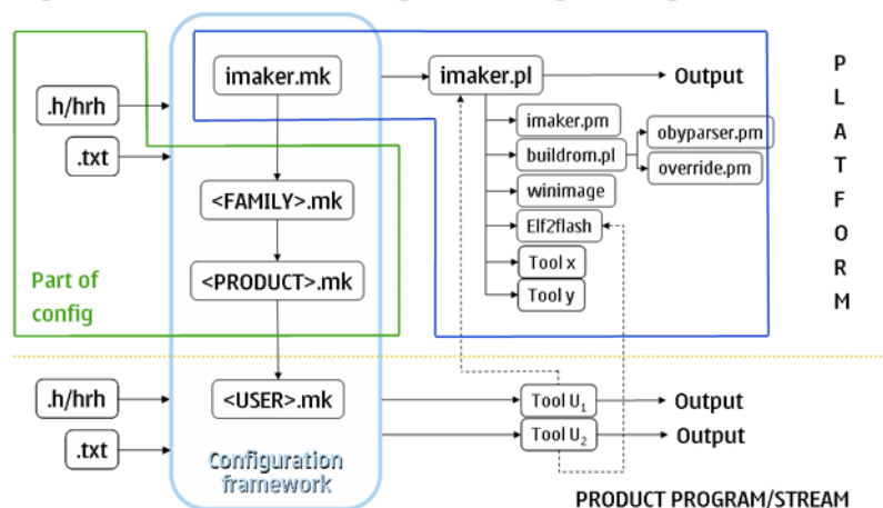
Figure 1: High-level architecture
